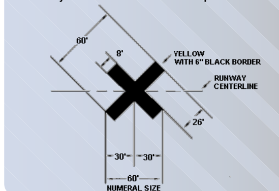
Runway "X" Closure Marker Detail & Specifications
